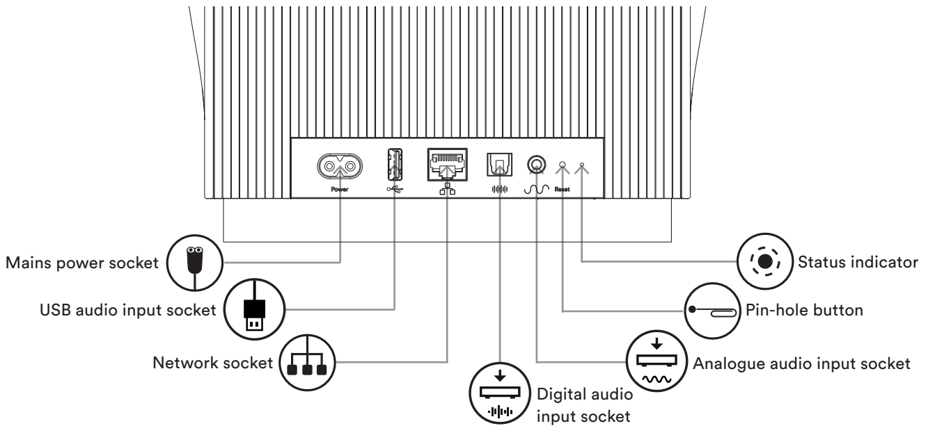
Diagram 3 – Mu-so Qb Mu-so Qb connection panel
